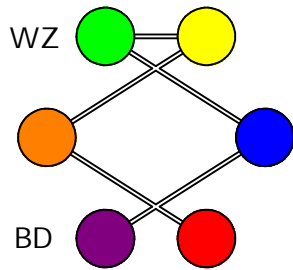
The order of Recursion
